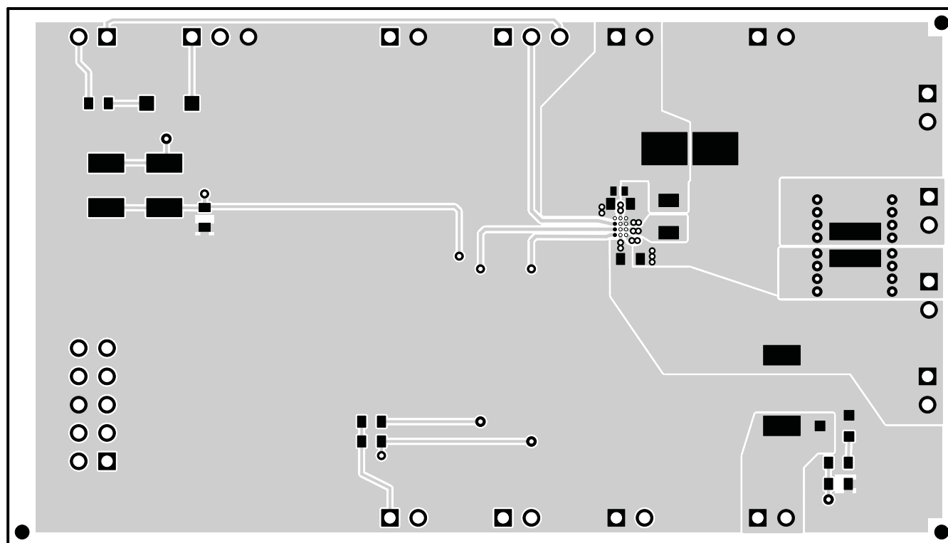
Figure 10. Top Layer
